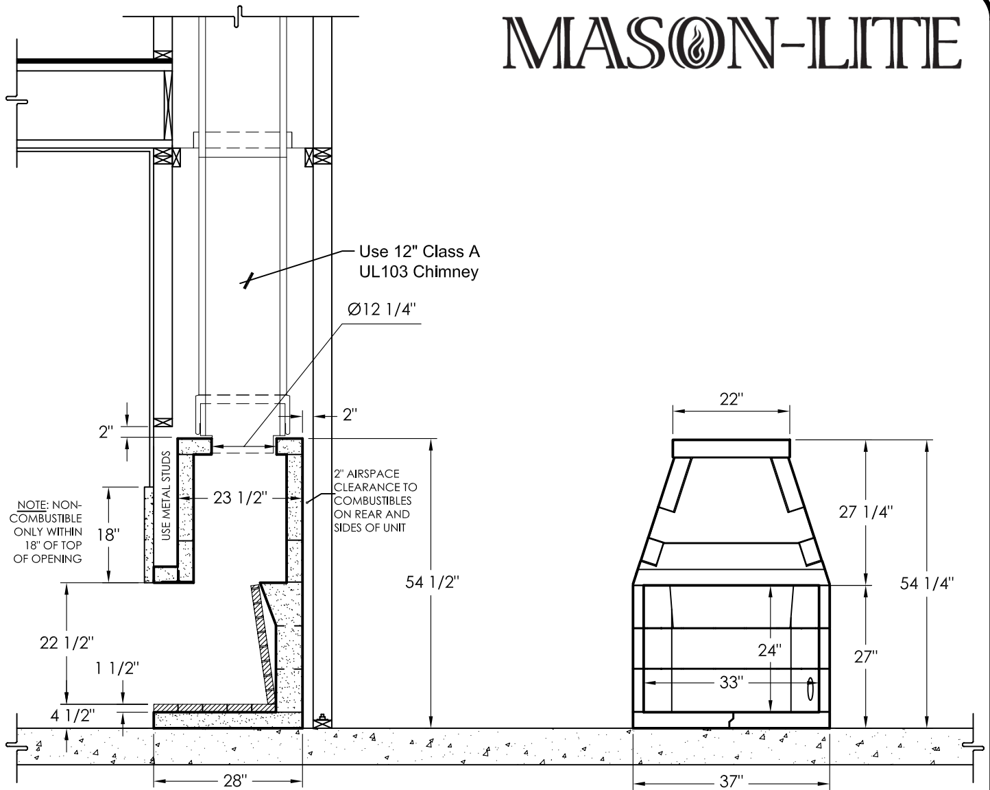
SECTION
