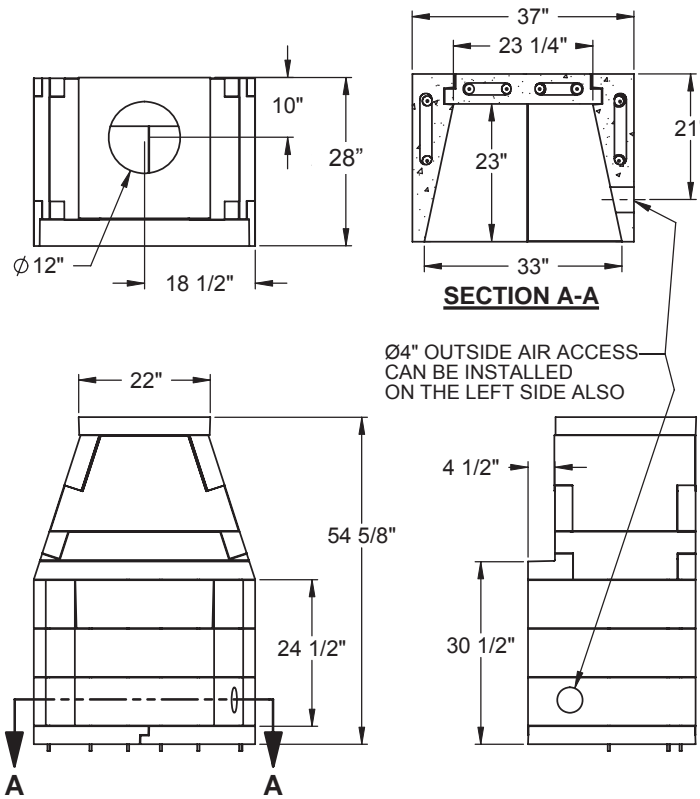
Mason-Lite MFP33 Fireplace Overall Dimensions
