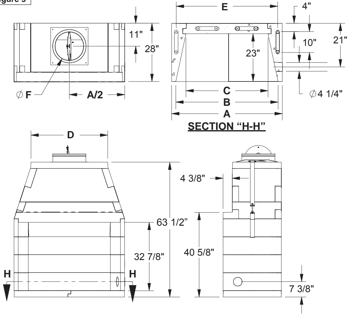
Mason-Lite MFP-39/44/49 Fireplace Overall Dimensions Figure 9
